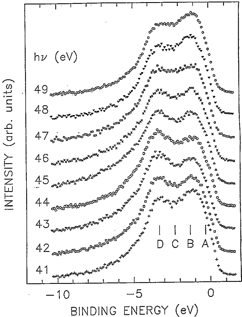
Figure 1. Valence-band spectra of the 1 Al 65 Cu 20 Ru 15 alloy measured for different photon energies h\nu around the Ru 4p→4d transition. A, B, C, and D identify binding energies for which CIS spectra were measured (figure 2).
